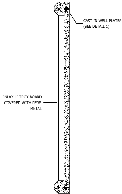
1 TYPICAL TOP AND BOTTOM EDGE
